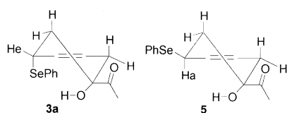
Figure 2. The conformation of 3a and 5 .
