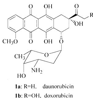
Figure 1. Structures of daunorubicin and doxorubicin.
